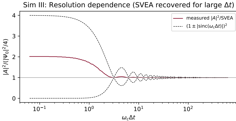
Figure 3: Simulation III. Demodulated intensity |A|^2 normalised by the SVEA value |\Psi_0|^2/4 , versus \omega_c \Delta t . The measured ratio (burgundy) stays within the exact boxcar envelope (1 \pm |\text{sinc}(\omega_c \Delta t)|)^2 (dashed) and converges to 1 (SVEA) for large windows.
