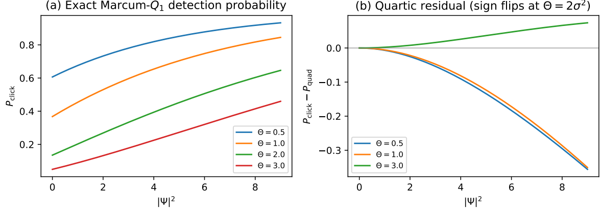
Figure 1: Simulation I. (a) Exact detection probability P_{\text{click}} versus |\Psi|^2 from the closed form (13) for four thresholds; the near-linear behaviour at small |\Psi|^2 is the Born rule. (b) Residual of P_{\text{click}} from a pure-quadratic fit, showing the quartic correction and its sign flip: negative (saturating) for \Theta = 0.5, 1.0 and positive for \Theta = 3.0 , with the crossover at \Theta = 2\sigma^2 .
