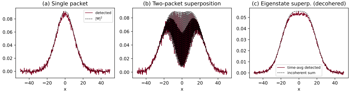
Figure 4: Simulation IV. Detected P_{\text{click}} - P_{\text{dark}} (burgundy) versus the relevant analytic target (dashed, scaled) for: (a) a single Gaussian packet ( |\Psi|^2 , r = 0.997 ); (b) a two-packet superposition (interference); (c) an energy-eigenstate superposition after time-averaging, matching the incoherent sum |c_1|^2|\phi_1|^2 + |c_2|^2|\phi_2|^2 ( r = 0.9992 ), i.e. decoherence.
