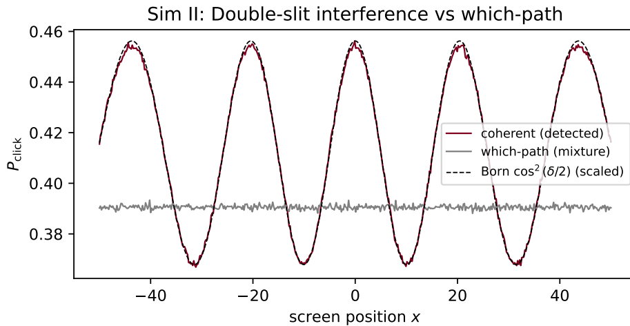
Figure 2: Simulation II. Detected P_{\text{click}} across the screen for the coherent two-path superposition (burgundy) versus the which-path statistical mixture (grey). The coherent case reproduces the \cos^2(\delta/2) fringes (dashed, scaled); the mixture is flat (fringes destroyed). Coherent-vs-Born correlation r = 0.9995 ; mixture modulation 1.7% of coherent.
